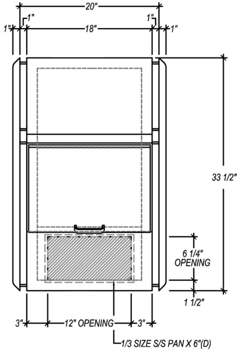
TOP VIEW
