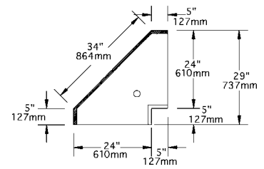
model #45ICWB-24
