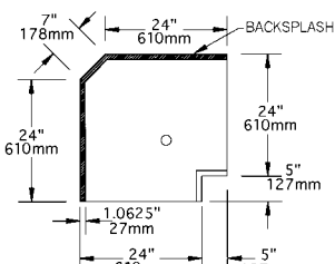
model #90ICWB-24
