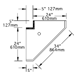
model #450CWB-24
