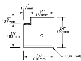
model #900CWB-19
