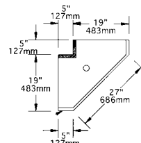
model #450CWB-19
