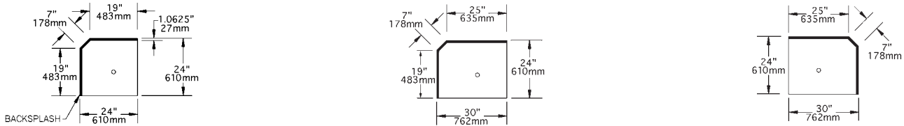
model #ICWB-24/24
