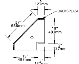
model #45ICWB-19
