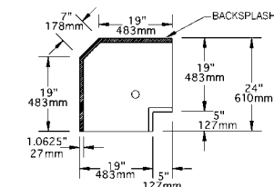
model #90ICWB-19
