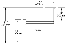
typical 19" (483mm) width elevation
